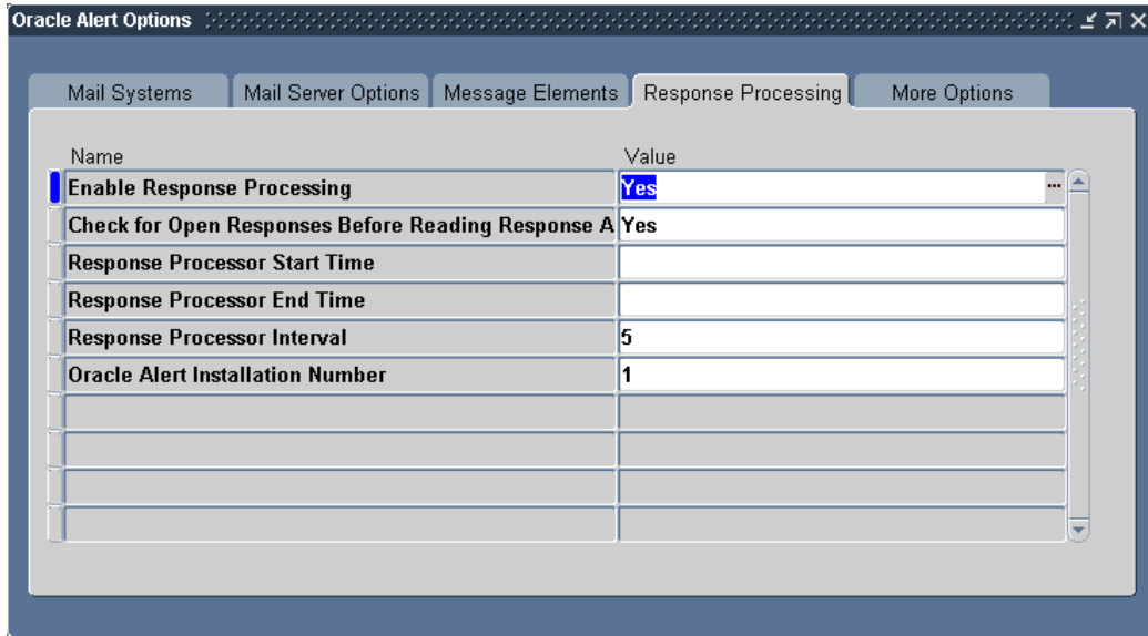
The Oracle Alert Options Window: Response Processing Tab
